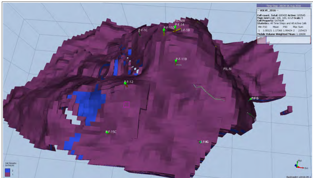
Figure 9.1: Volve Full Field Model SATNUM Array
